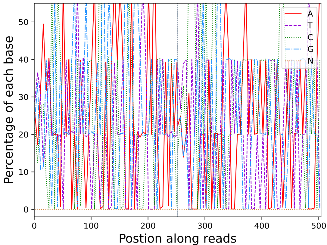
Base percentage along reads (R10919)
